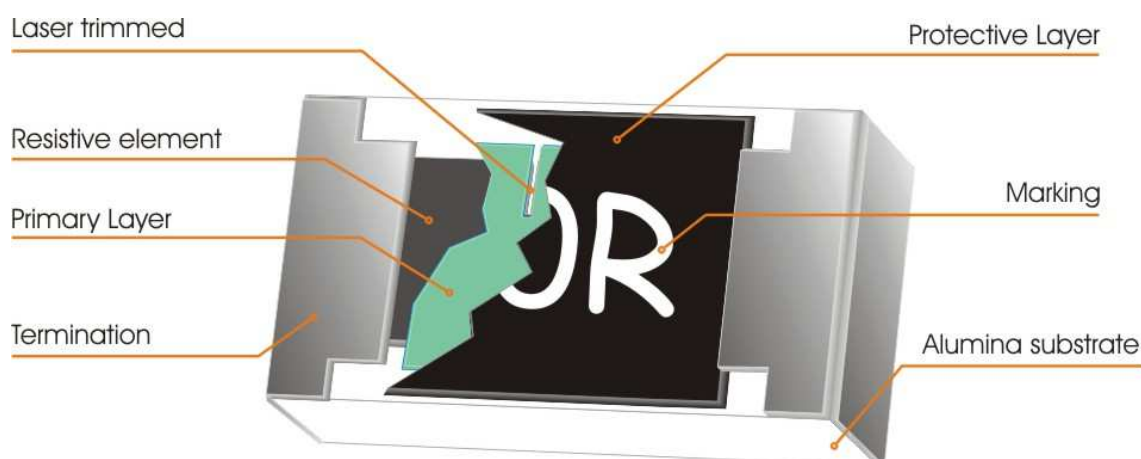
Fig 1. Construction of Chip-R ATSXX
