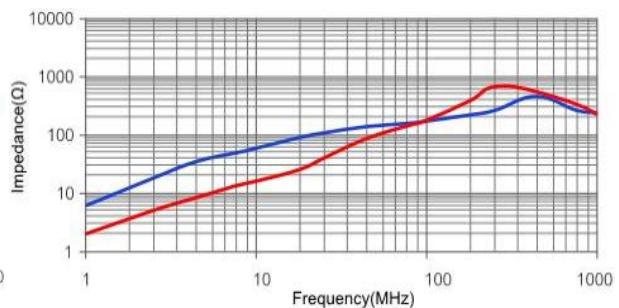
ALCM4520M151T
