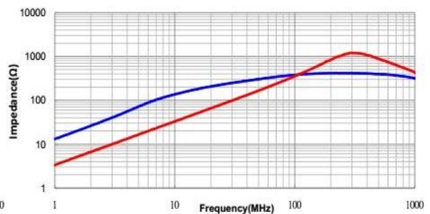
ALCM4520M421T
