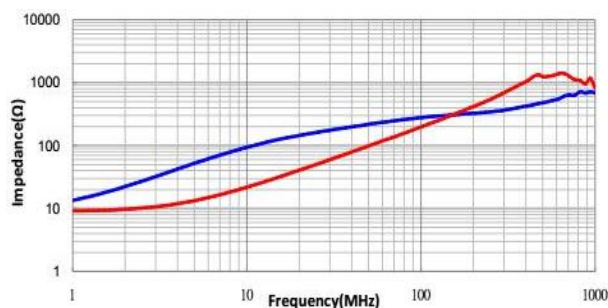
ALCM4520M231&301T
