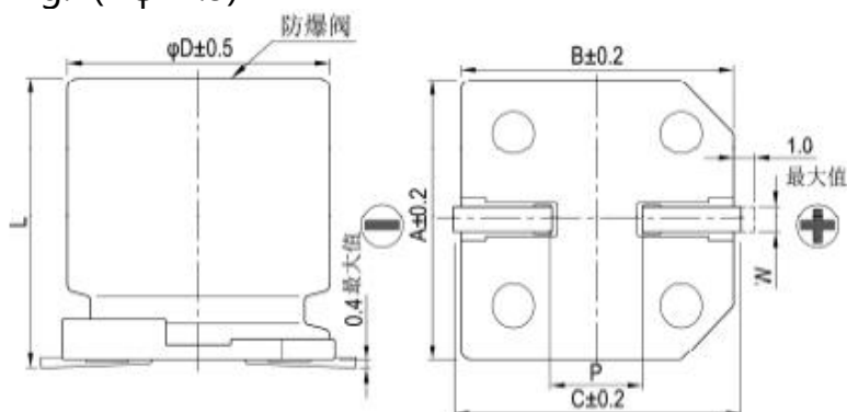
Fig.2( \geq \phi 12.5 )
