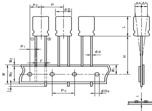
Taping dimension
