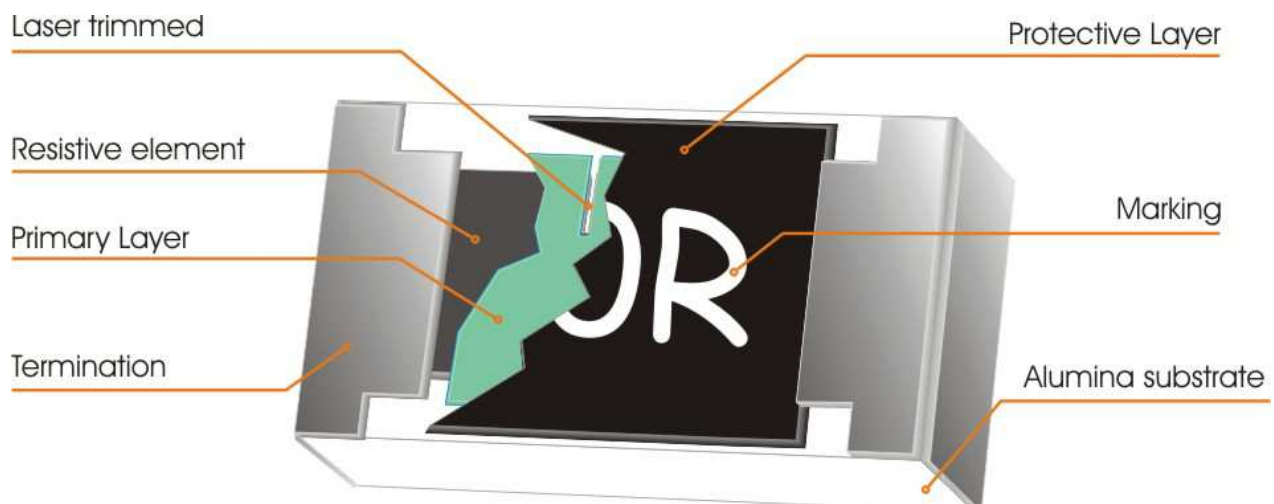
Fig 1. Construction of Chip-R ARQ
