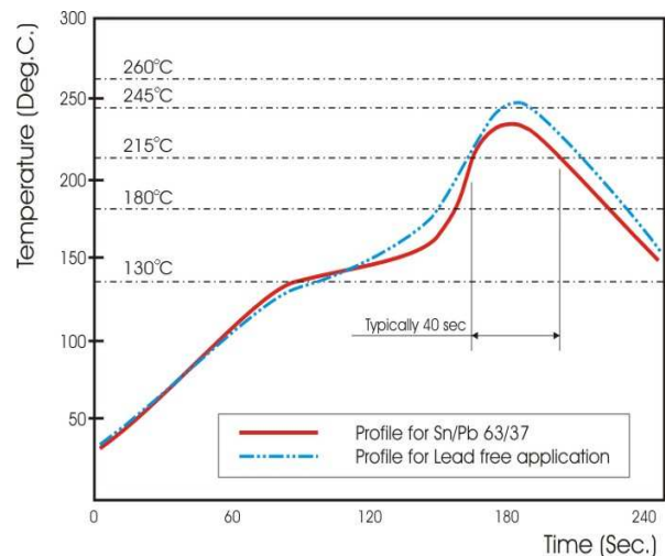
Fig 3. Infrared soldering profile for Chip Resistors CR02
