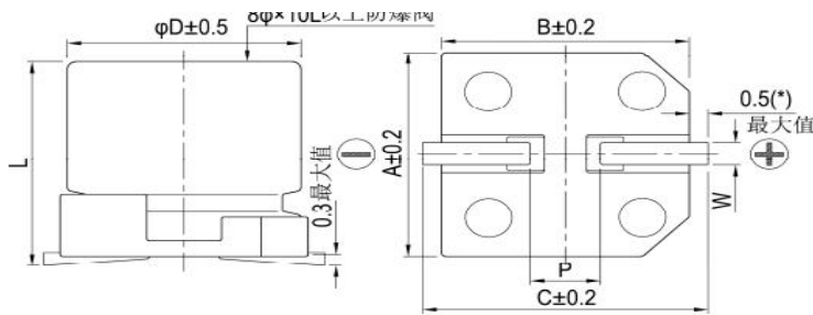
尺寸: Dimensions (Unit: mm)
